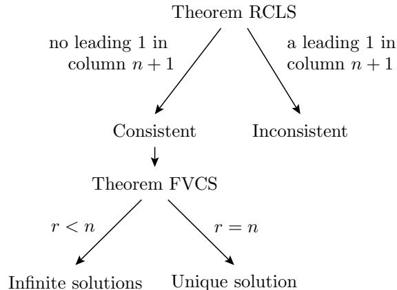
Diagram DTLS. Decision Tree for Solving Linear Systems
