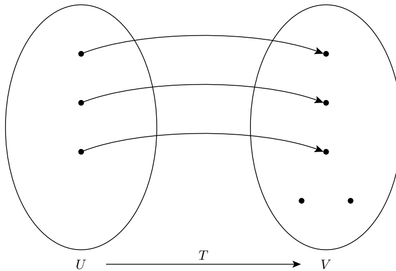
Diagram ILT. Injective Linear Transformation
