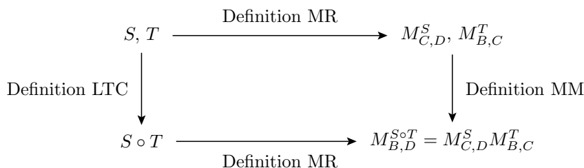
Figure MRCLT. Matrix Representation and Composition of Linear Transformations
