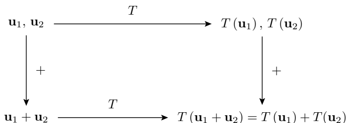
Diagram DLTA. Definition of Linear Transformation, Additive
