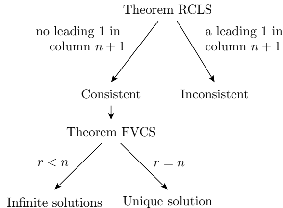
Diagram DTSLs. Decision Tree for Solving Linear Systems
